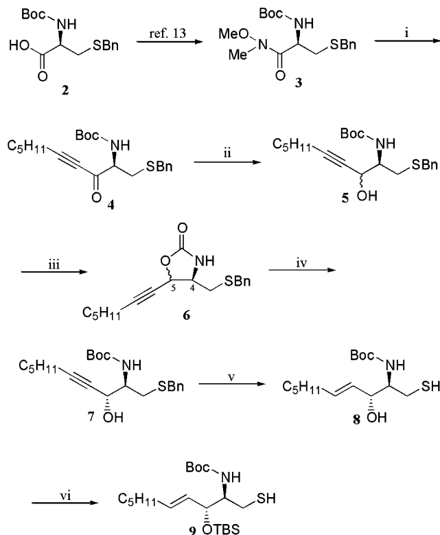
Scheme 1. (i) \text{C}_5\text{H}_{11}\text{CCl} , THF, -43\text{ }^{\circ}\text{C} ; (ii) \text{LiAl}(\text{O}i\text{Bu})_3\text{H} , EtOH, -78\text{ }^{\circ}\text{C} ; (iii) NaH, THF, 50\text{ }^{\circ}\text{C} ; (iv) (a) \text{Boc}_2\text{O} , DMAP, \text{Et}_3\text{N} , DMF, 0\text{ }^{\circ}\text{C} ; (b) separation; (c) \text{Cs}_2\text{CO}_3 , MeOH, 47% for six steps; (v) Li, liq. \text{NH}_3 , THF, reflux, 93%; (vi) (a) TBSCl, DMAP, \text{Et}_3\text{N} , DMF, 73%; (b) TBAF, THF, -78\text{ }^{\circ}\text{C} , quant.
