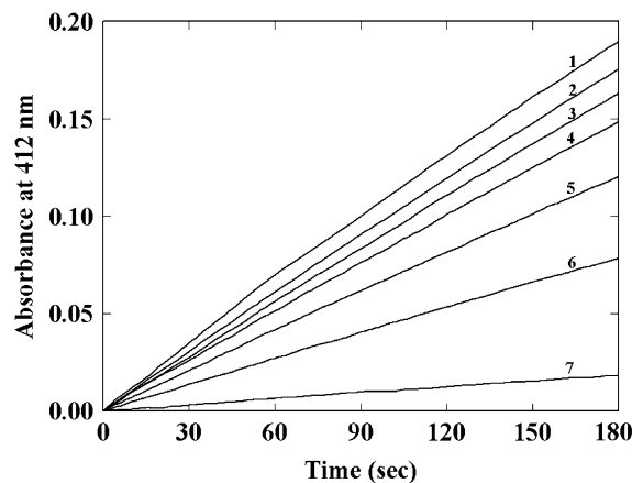
Figure 3. Enzymatic hydrolysis of mixed micelle of sulfur analogue 1 with Triton X-100 (the molar concentration of 1:10) by B. cereus SMase. The analogue concentrations: (1) 1.6; (2) 1.2; (3) 1.0; (4) 0.8; (5) 0.6; (6) 0.4; (7) 0.2 mM.
