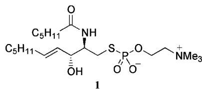
Figure 2. Designed sulfur analogue of sphingomyelin.
