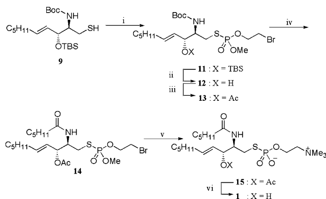
Scheme 2. (i) B , \text{CBr}_4 , pyr, 0^\circ\text{C} , quant.; (ii) 2N HCl, MeOH; (iii) \text{Ac}_2\text{O} , pyr; (iv) TFA, \text{CH}_2\text{Cl}_2 , then 1N NaOH, \text{C}_5\text{H}_{11}\text{COCl} , 88%; (v) \text{Me}_3\text{N} , toluene, 95%; (vi) KOH, MeOH, 90%.
